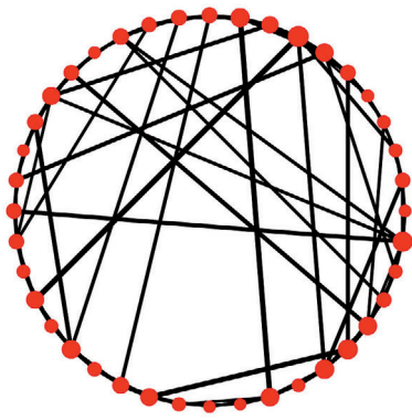
Figure 1. Node and edge betweenness in a model of small-world networks. Undirected edges (black lines) connect nodes (red dots). Betweenness measures how central each node and edge is to the shortest network paths connecting any two nodes. In this plot, node diameter and edge thickness are proportional to node and edge betweenness, respectively.
