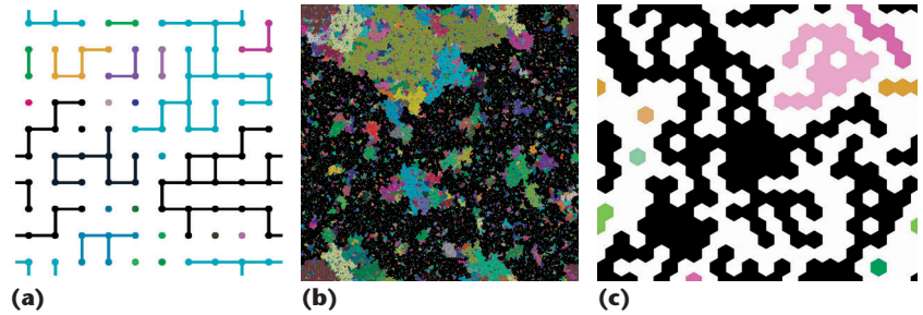
Figure 2. Two instances of bond-percolation on a 2D square lattice, and an instance of site-percolation on a triangular lattice. In bond-percolation, neighboring lattice points are connected with probability p , and connected clusters in the resulting network are identified via breadth-first search. Separate clusters are colored distinctly, for (a) a 10 \times 10 grid and (b) a 1,024 \times 1,024 grid. In (c) site-percolation, lattice sites are filled with probability p , and clusters connect the filled neighboring sites.
