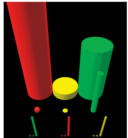
Figure 4. Snapshot in the stochastic time evolution of the Repressilator. Protein concentrations (back row), mRNA concentrations (middle) and promoter states (front) are shown. At this instant, TetR (red) concentration is high, leading to suppression of \lambda cl (yellow). Because \lambda cl is low, however, Lacl (green) concentration can grow, leading to TetR's eventual suppression.
