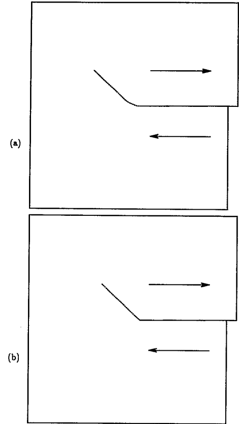
FIG. 5. Qualitative picture of crack growth in mode II, where the crack curves so as to reduce the mode-II stress, leaving only mode-I stress. (a) Our picture, where the crack curves gradually to the direction where K_{II}=0 , on a length scale of 2v/(fK_I) . (b) The "principle of local symmetry" picture, where there is a sharp kink to the direction where K_{II}=0 . Note that in the f \rightarrow \infty limit, the two pictures agree.
