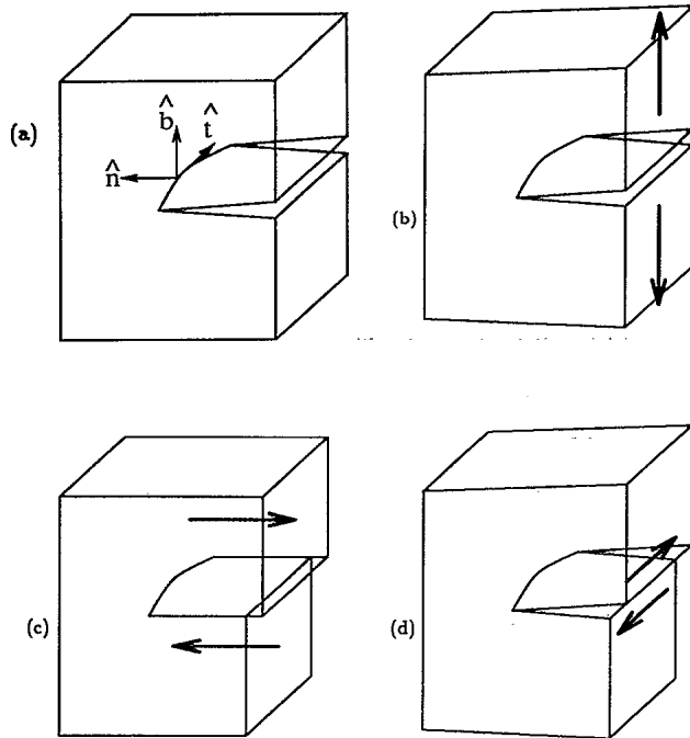
FIG. 1. (a) Vectors associated with a point on the crack front: \hat{\mathbf{t}} is the tangent to the crack-front curve; \hat{\mathbf{n}} , perpendicular to \hat{\mathbf{t}} and in the crack plane, is the direction of crack growth; \hat{\mathbf{b}} \equiv \hat{\mathbf{t}} \times \hat{\mathbf{n}} is the normal to the crack plane. (b) A crack loaded in mode I, with K_I > 0 . Arrows show direction of crack opening displacement. (c) A crack loaded in mode II, with K_{II} > 0 . (d) A crack loaded in mode III, with K_{III} > 0 .
